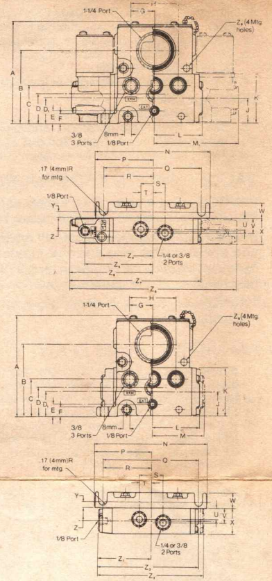
DIMENSIONAL DATA
