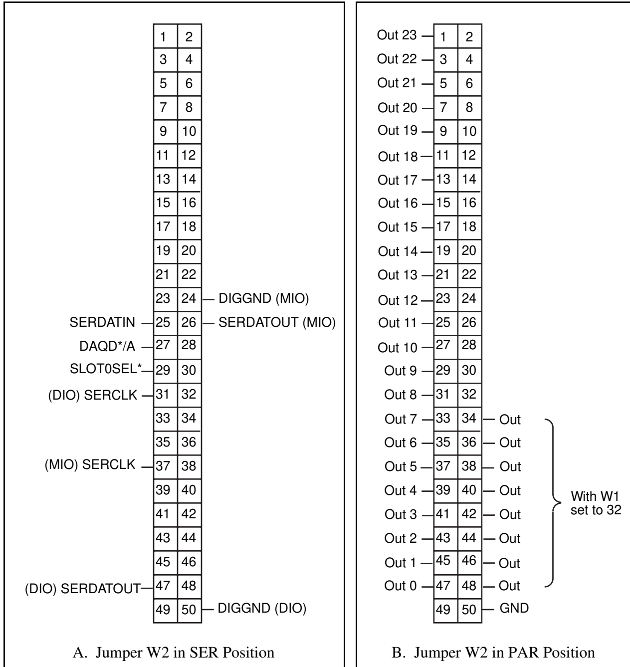
Figure 3-3. SCXI-1162HV Rear Signal Connector Pin Assignments
